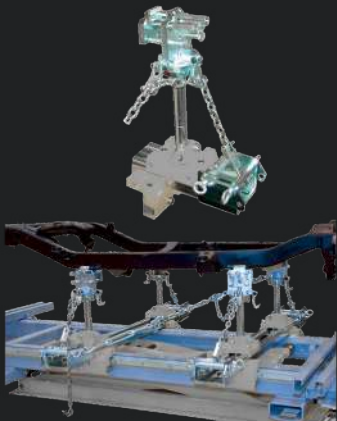
Truck clamps
