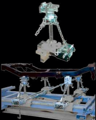
Truck clamps
